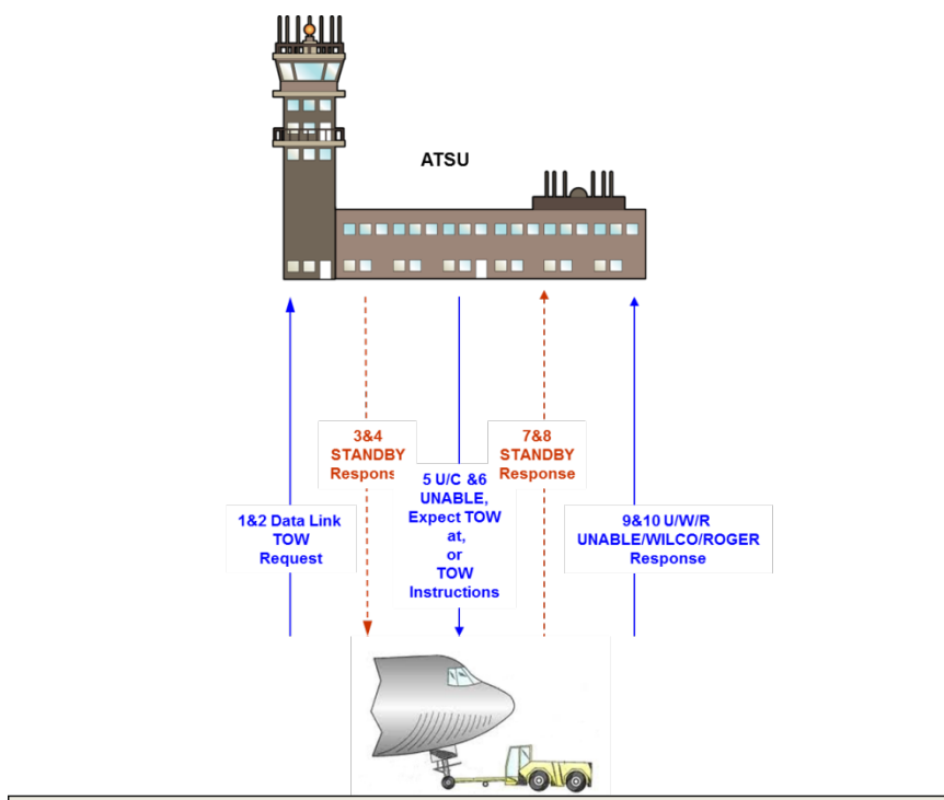
Figure 31: Data Link TOW Request Operating Method Diagram
